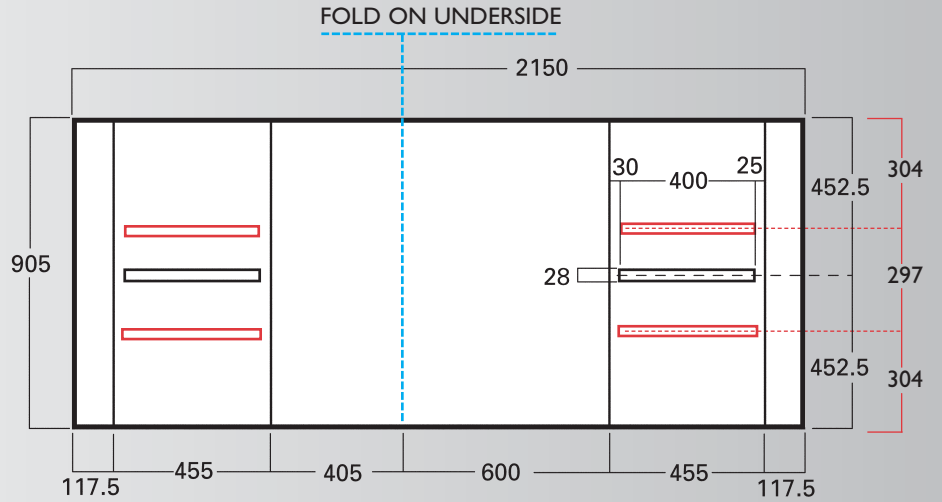
GRAPHIC SIZE FOR ONE AND TWO SHELF UNIT
