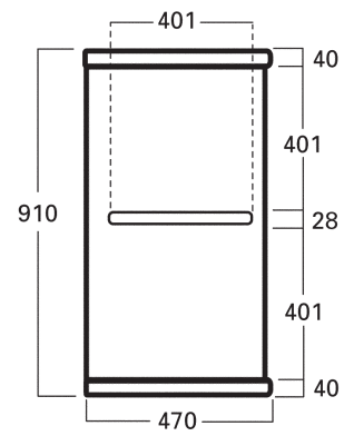
SIDE - ONE SHELF
