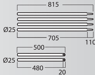
POLES - M ROOF KIT STYLE
