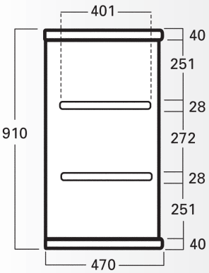
SIDE - TWO SHELVES
