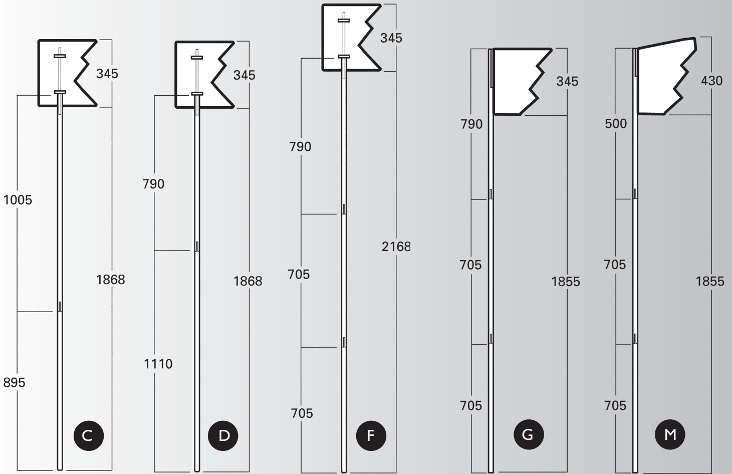
Single sided foam board headers with plastic poles, clips and screwed through fixings.
