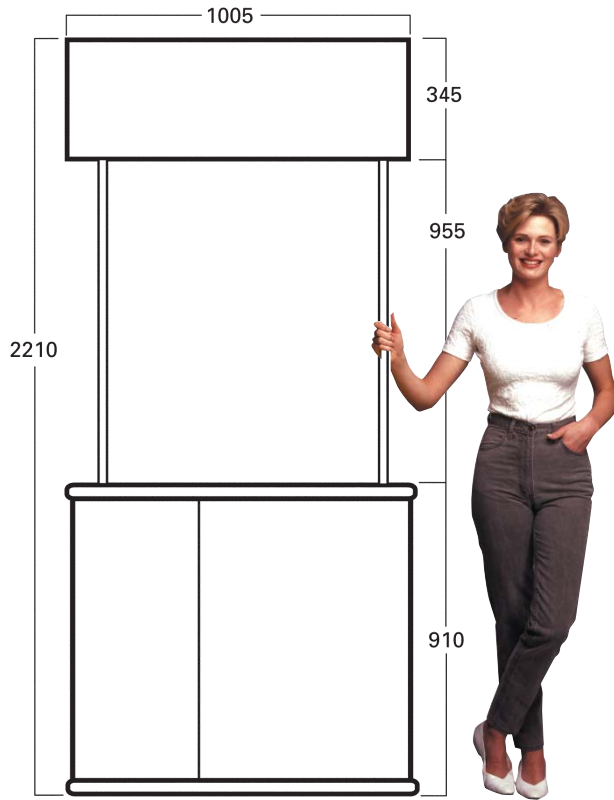
UNIT AND HEADER
