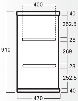
SIDE - TWO SHELVES
