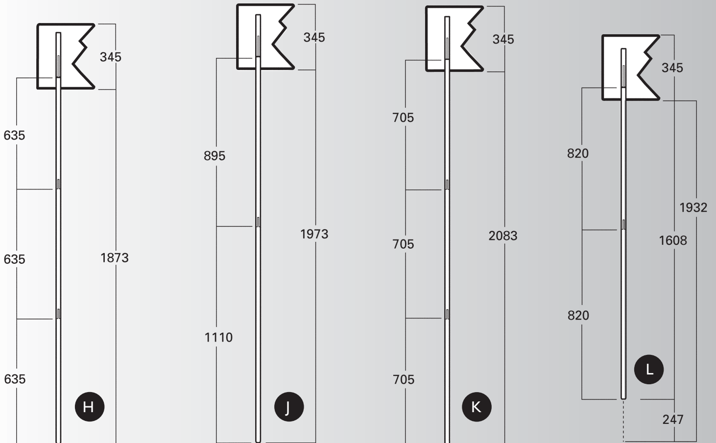
Pole set raised from ground as poles sit on baseshelf.
