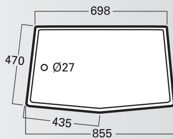
ORIGINAL TOP / BOTTOM
