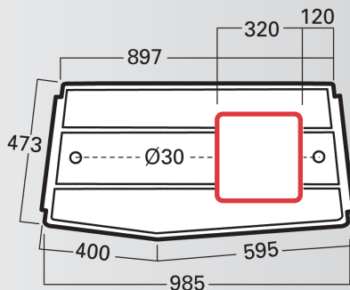
SHELF WITH BIN
