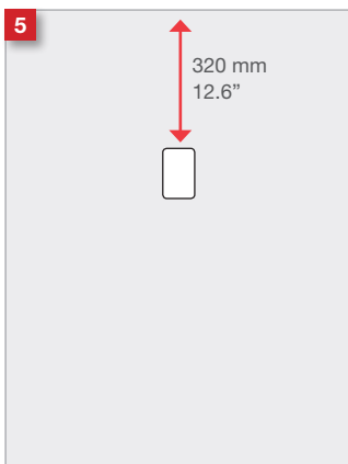
Make a 80x130 mm / 3.2x5.3" hole in the panel, located 320 mm / 12.6" from the top in the center of your panel.
